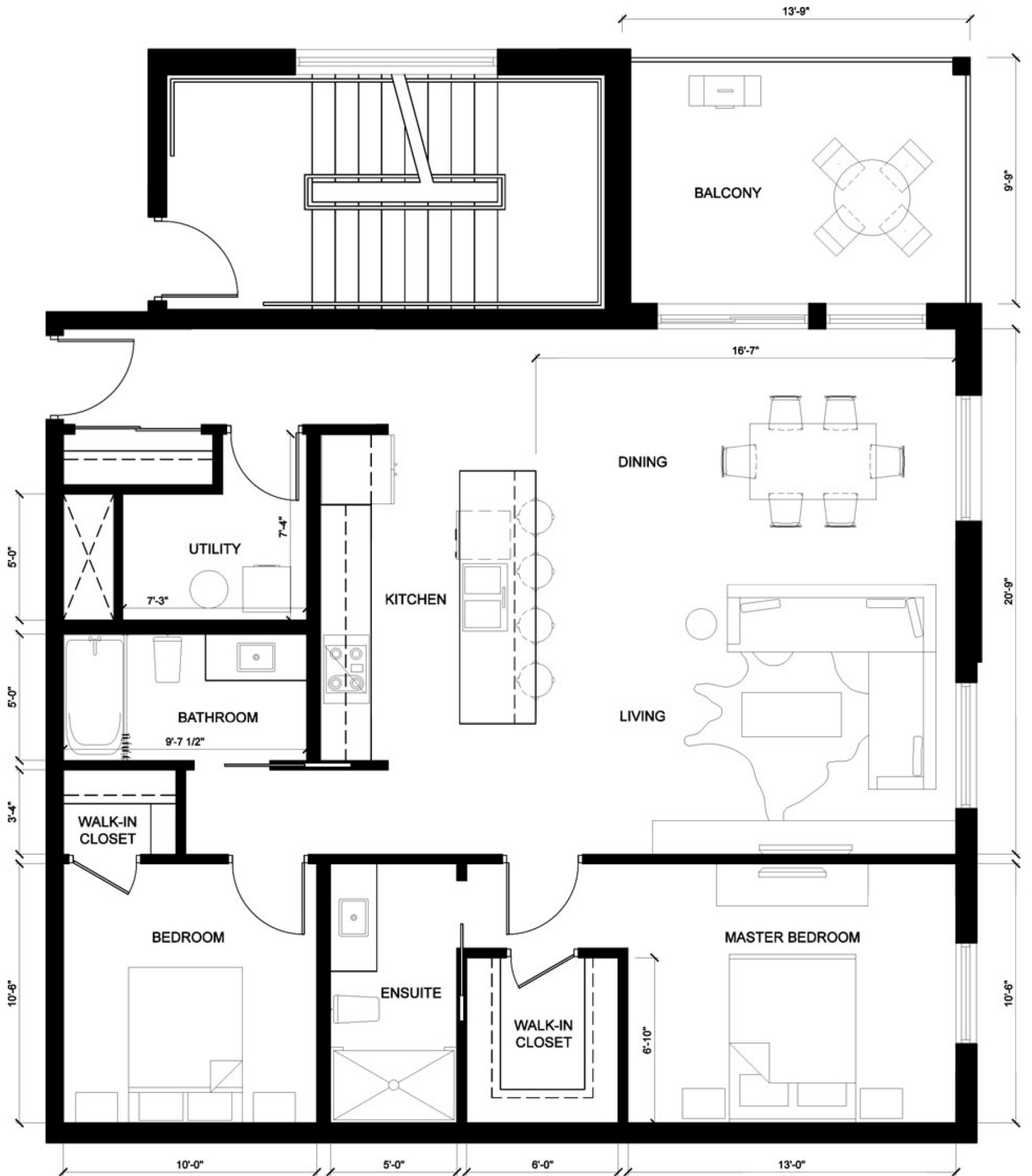
THIRD FLOOR
